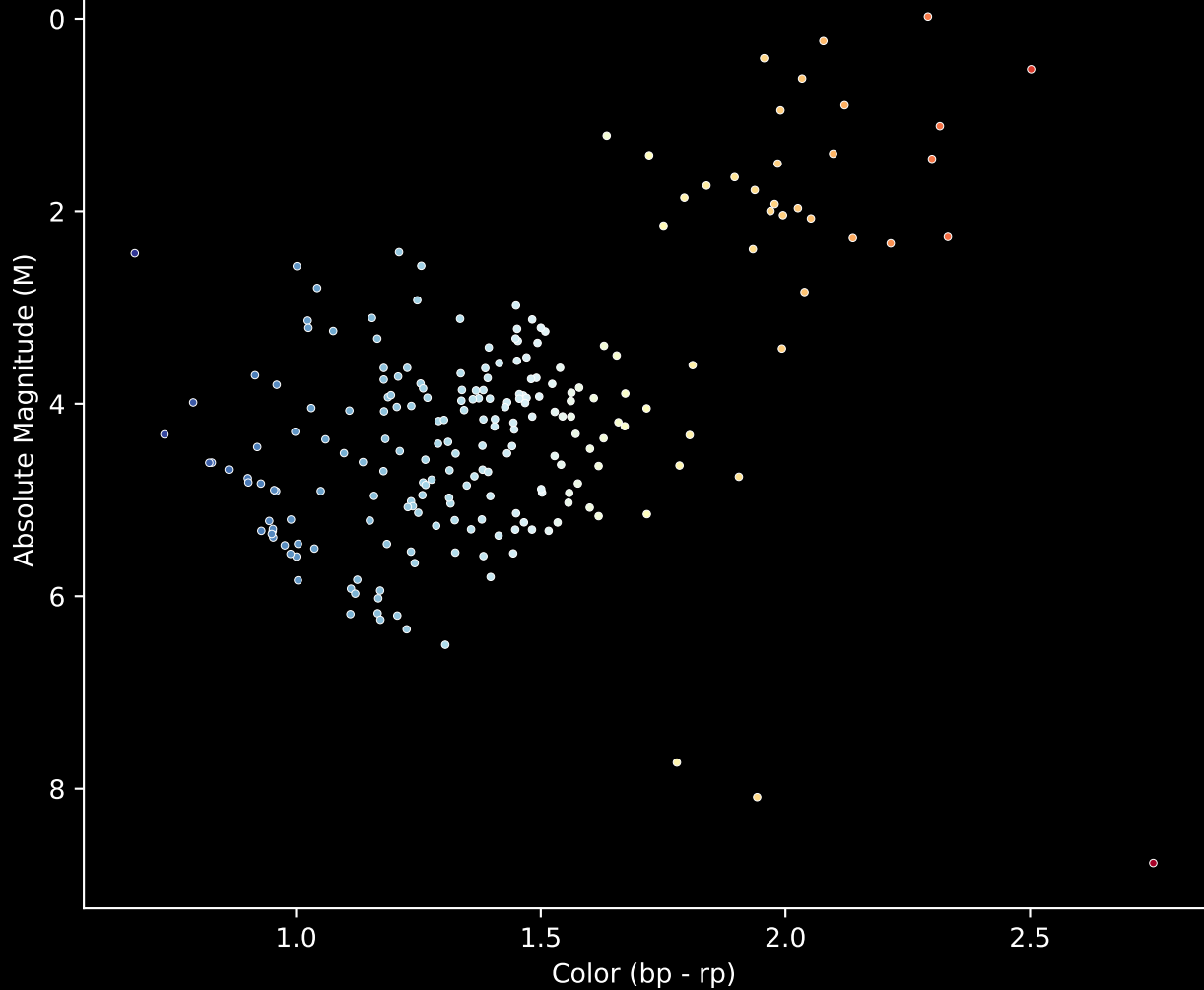
GALAH DR4 Field [3669] Stars ( n = 221 ) Hertzsprung-Russell Diagram
