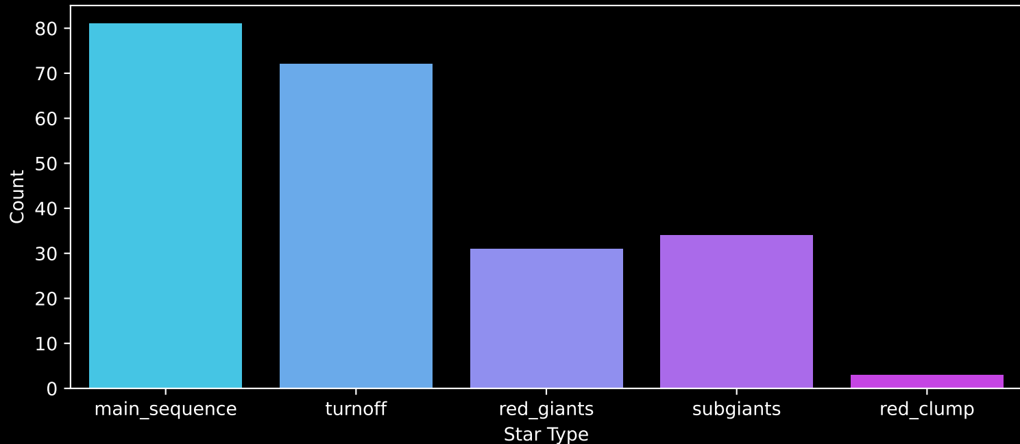
GALAH DR4 Field: [3669] Count plot of Star Type
