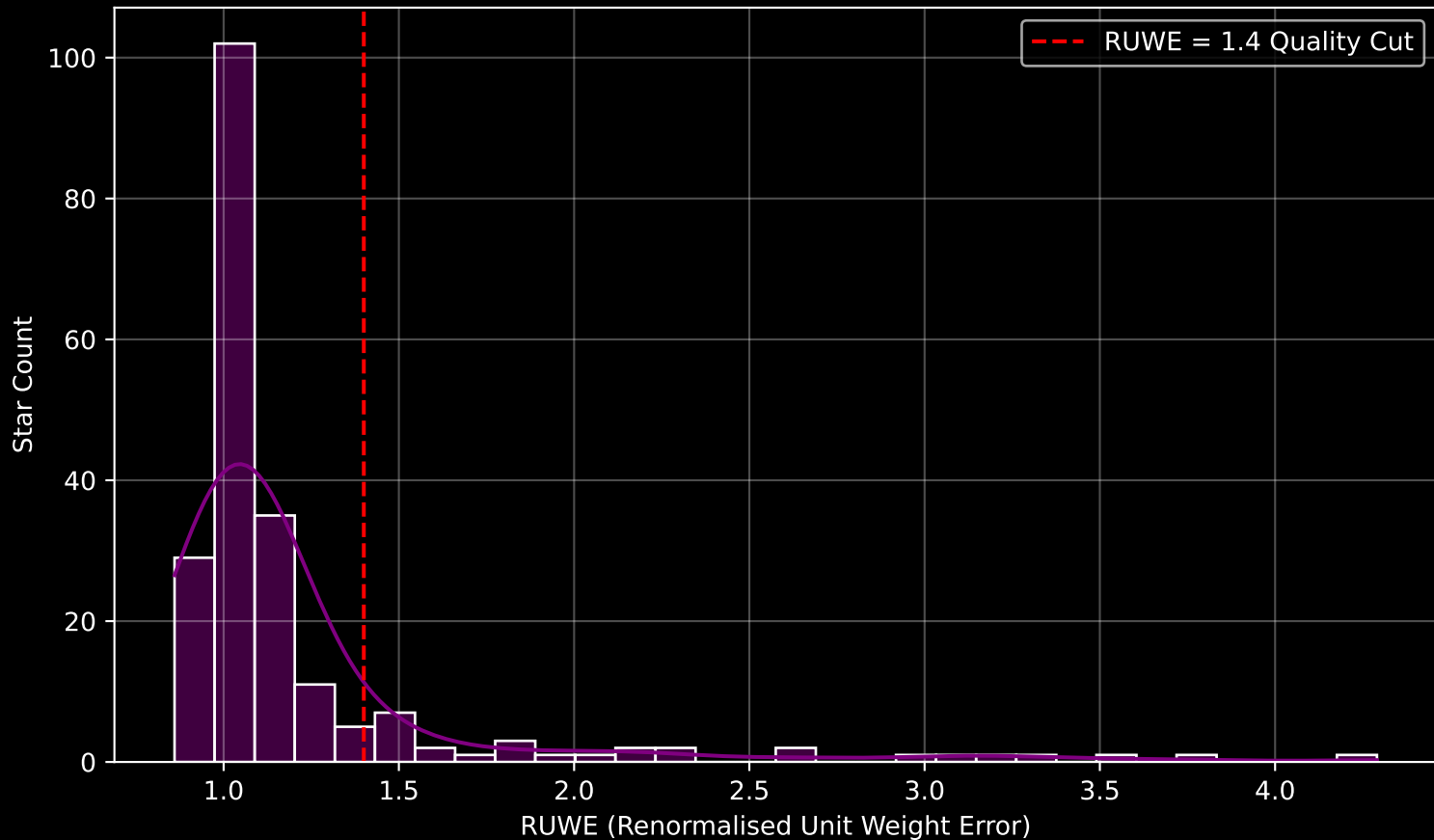
GALAH DR4 Field [3669] RUWE Distribution (n= 210)
