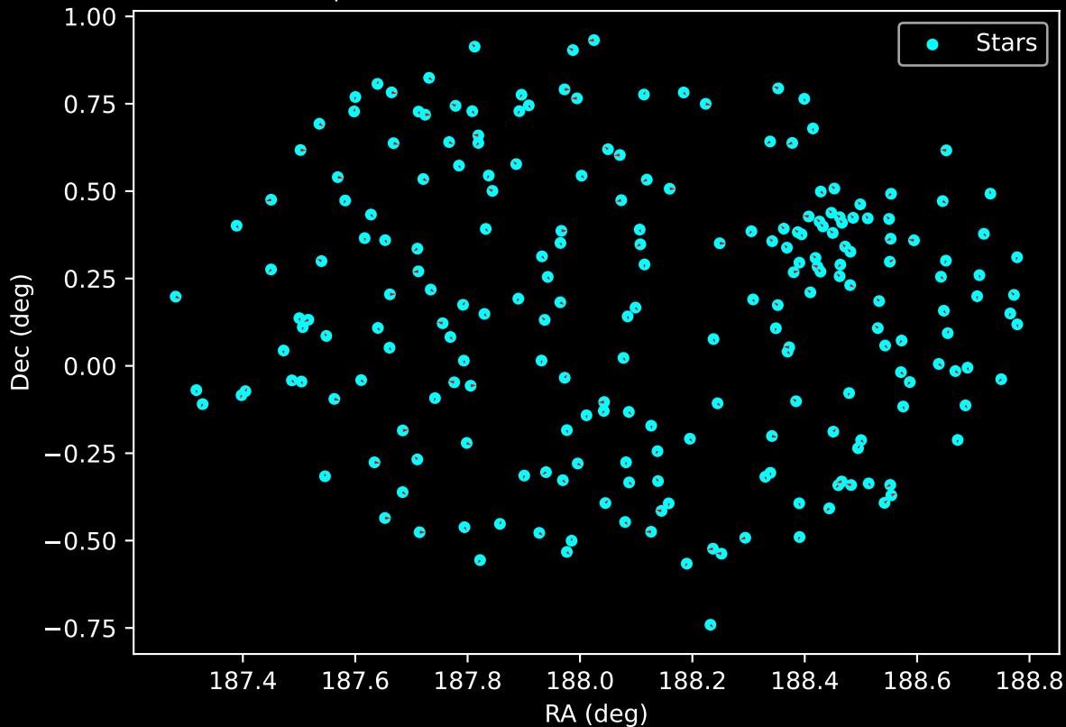
GALAH DR4 Field: [3669] Proper Motion Vectors for Gaia Star Field (n= 221)
