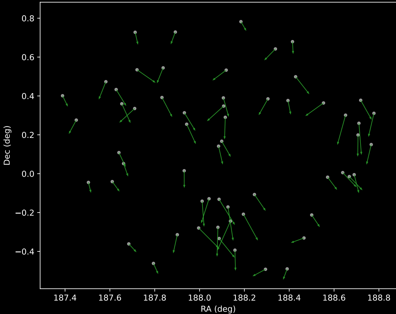
GALAH DR4 Cluster 4 Proper Motion Vectors (n=59)
